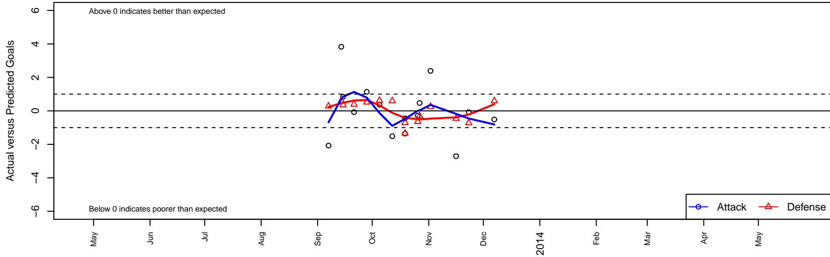
Legends FC FI1 G01 Dots are actual minus expected GF (blue circles) and GA (red triangles). Blue line is smoothed change in attack strength. Red is smoothed change in defense strength.
